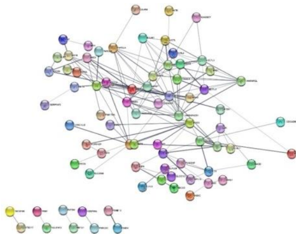
Figure 3: Protein-Protein Interaction network constructed with DEGs. The nodes represents proteins while the edges represent the protein-protein associations.
