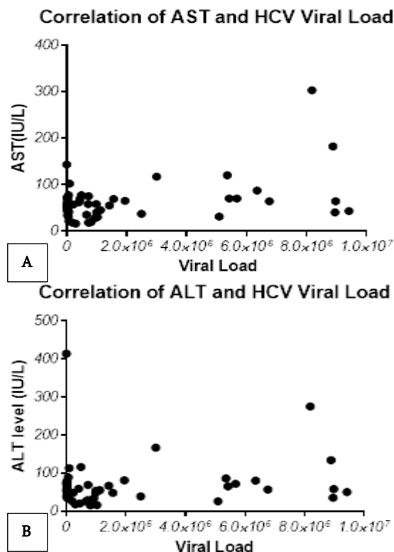
Figure 5: Correlation of HCV viral load with ALT (Pearson correlation coefficient r=0.15 , p value=0.28) and AST (Pearson correlation coefficient r=0.42 , p value=0.002). A positive association has been observed between the levels of AST, ALT and viral load. It indicates the increase in hepatitis C viral load, the level of ALT and AST also raises.
